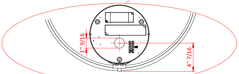
Mounting Center
